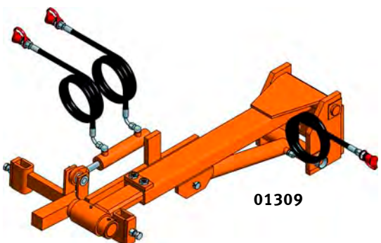
Telescopic hydraulic lift with side slope adjustment (hydraulic) with hydraulic hoses and connectors right
