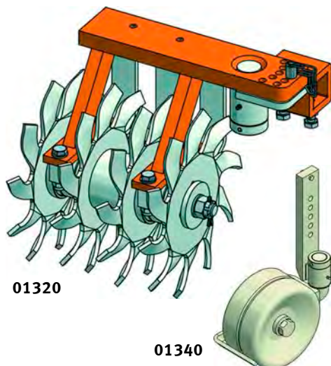
Rotary star tiller with four star wheels for orchards
